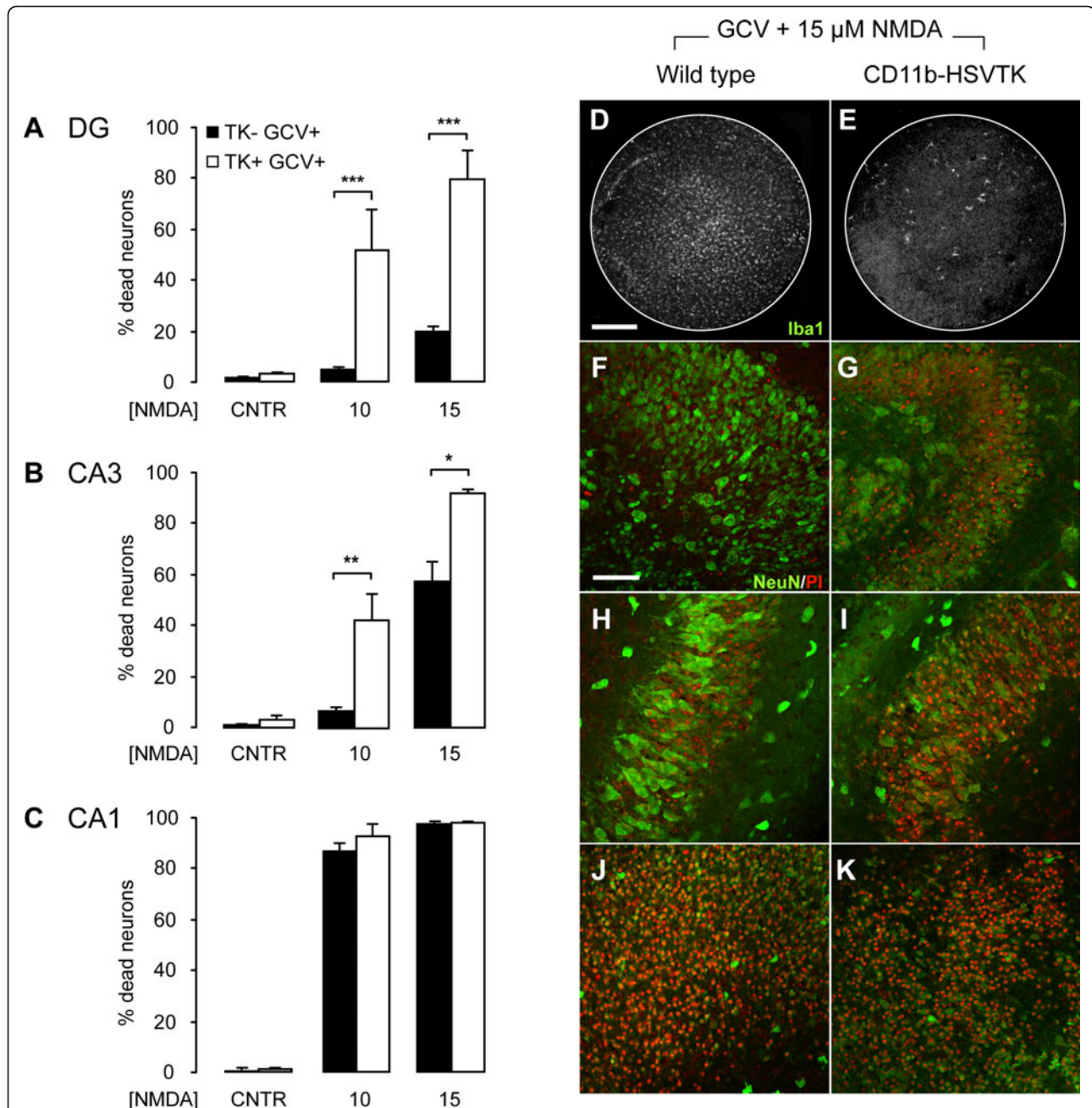
Figure 5 Microglial depletion in CD11b-HSVTK slice cultures by ganciclovir treatment also results in a strong increase in neuronal cell death in response to excitotoxicity. Graphs represent the percentages of neuronal cell death per hippocampal region (A to C) in response to 0, 10, and 15 \mu M NMDA in wild type (TK- GCV+) and microglia-depleted CD11b-HSVTK slice cultures (TK + GCV+). Microglial depletion alone did not lead to a significant increase in neuronal cell death (A-C; CNTR). However, in the absence of microglia, neuronal cell death in response to NMDA-induced excitotoxicity was severely enhanced in the DG (A) and CA3 (B). Almost no microglia cells were present when TK slices were treated with GCV (E) compared to wild type slice cultures (D). Confocal images clearly show the effect of microglial depletion on neuronal degeneration in response to 15 \mu M NMDA (F-K). Here, in the absence of microglia, neuronal cell death was significantly increased in the DG from 19.5% to 79.2% (F,G) and in the CA3 from 56.6% to 90.3% (H, I). In the CA1 (J,K) no significant effect in response to 15 \mu M NMDA was observed between wild type and TK slice cultures (96.2% versus 96.6%, respectively). Data are a summary of three individual experiments with at least 6 slice cultures per condition. Bars indicate mean \pm SEM. * p < 0.05, ** p < 0.01, *** p < 0.001, ANOVA. Scale bars indicate 300 \mu M (D,E) and 75 \mu M (F-K).
