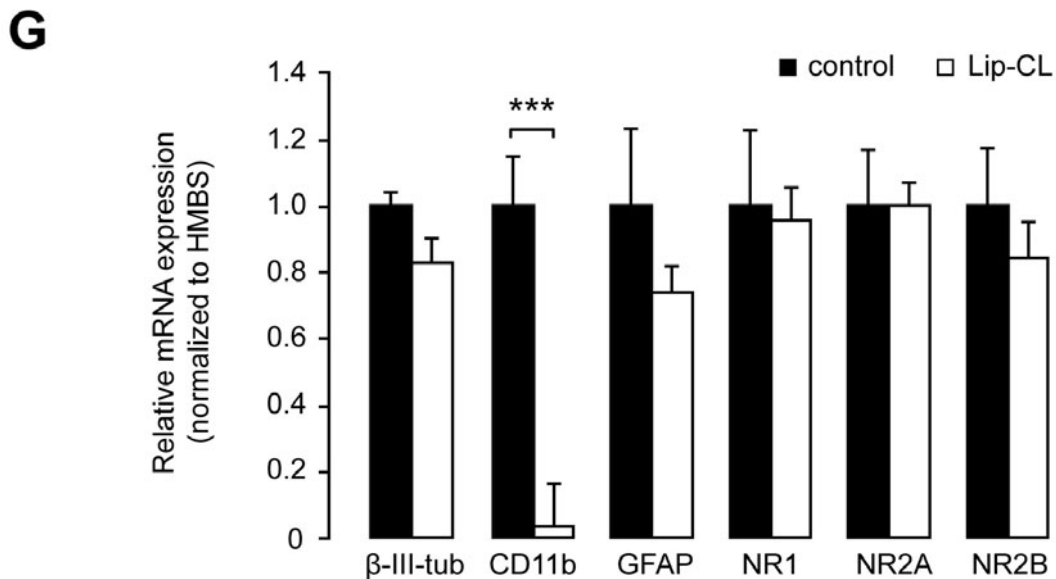
Figure 3 Liposomal clodronate specifically depletes microglia from hippocampal slice cultures. Untreated mouse hippocampal slice cultures showed preserved organotypic structure with ramified microglia (A, Iba1), astrocytes (B, GFAP) and neuronal layers CA1/CA3/DG (C, NeuN). Overnight treatment with liposome-encapsulated clodronate (Lip-CL) directly after slice culture preparation resulted in specific depletion of microglia (D), while astrocytes (E) and neurons (F) remained unaffected. After 6 days in culture, the microglia population in Lip-CL treated slice cultures was reduced to less than 5% (D). Scale bars indicate 300 \mu M (overviews) and 25 \mu M (inserts). Confocal images were grey-scaled. (G) qPCR analysis of control- and Lip-CL-treated slice cultures revealed no differences in the levels of \beta -III-tubulin and GFAP confirming our observation that Lip-CL does not affect the presence of neurons and astrocytes. In comparison, CD11b mRNA levels were strongly reduced in Lip-CL-treated slice cultures, indicating that the number of endogenous microglia left in these slice cultures is really low. Finally, no differences were observed in NR1, NR2A and NR2B subunit mRNA levels, showing that these were not affected by the Lip-CL treatment. Bars indicate mean \pm SEM. *** p < 0.001 .
