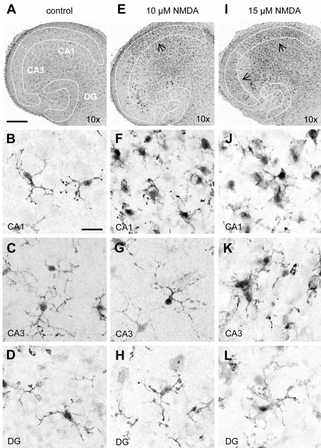
Figure 2 Microglial activation coincides with selective neuronal vulnerability towards excitotoxicity. Confocal images of microglia in control (A-D), 10 \mu M (E-H) and 15 \mu M (I-L) NMDA-treated slice cultures, as determined by Iba1-immuno-histochemistry. After 6 days in culture (A), microglia were evenly distributed throughout the slice cultures and displayed a typical ramified morphology (B:CA1, C:CA3, D:DG). At 10 \mu M NMDA (E), changes in the CA1 region were clearly visible as numerous microglia accumulated at the site of injury (E, arrow). Morphologically, these microglia displayed an "activated" phenotype (F, CA1) with enlarged somata and loss of secondary and tertiary branching. In contrast, accumulation of microglia did not occur in the CA3 (G) and DG (H) and these cells retained their ramified phenotype. At 15 \mu M NMDA, pronounced accumulation of morphologically activated microglia (I, arrows) was observed in both CA1 (J) and CA3 (K). In contrast, microglia in the DG (L) showed only mild activation and accumulation of microglia was minimal in this region. Scale bars indicate 300 \mu M (overviews) and 25 \mu M (magnifications). Confocal images were gray-scaled and inverted.
